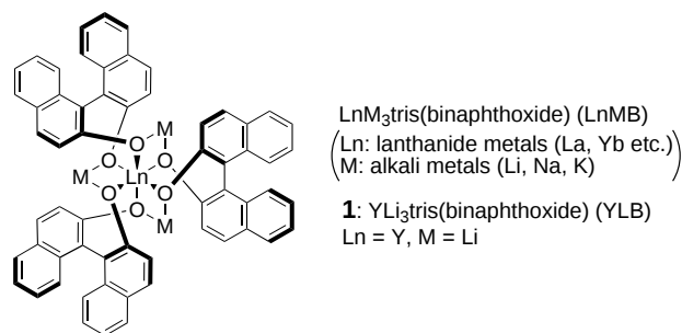
Scheme 1. Structure of heterobimetallic [\text{LnM}_3\{\text{tris}(\text{binaphthoxide})\}] and 1 (Ln = Y, M = Li).
